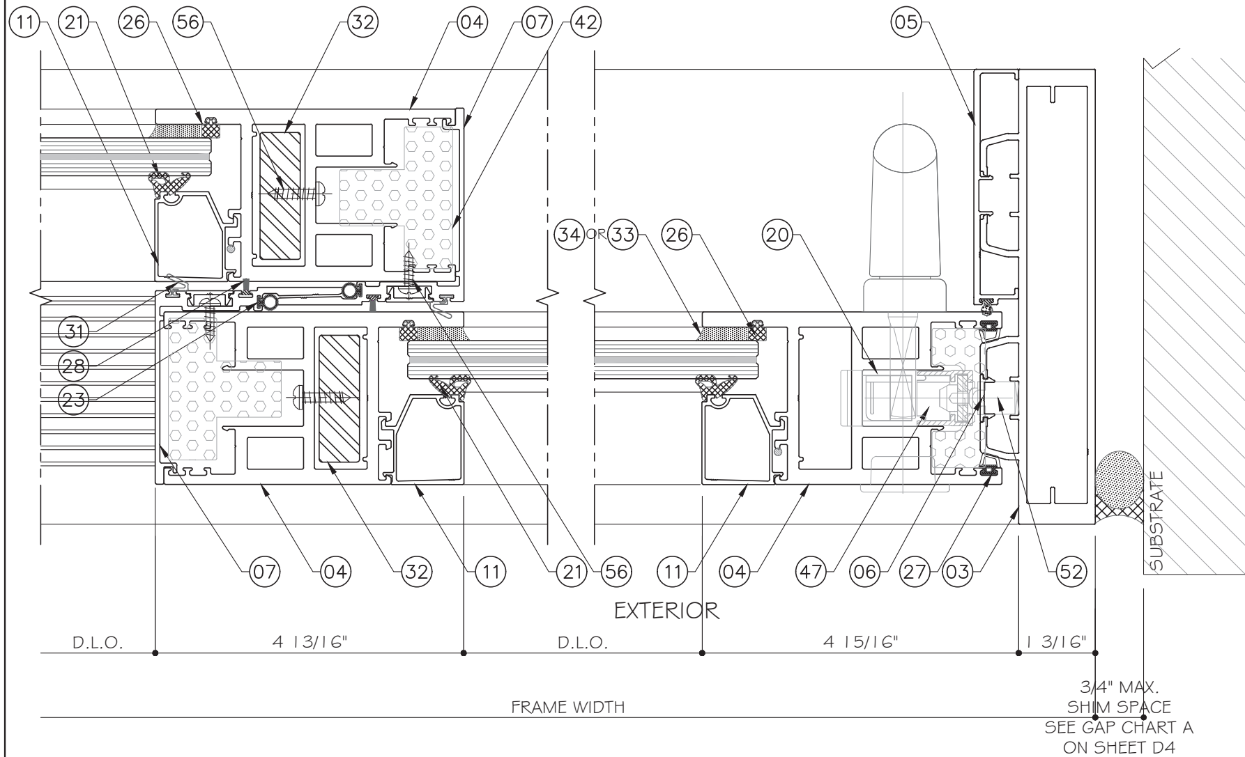
H D3 DETAIL
