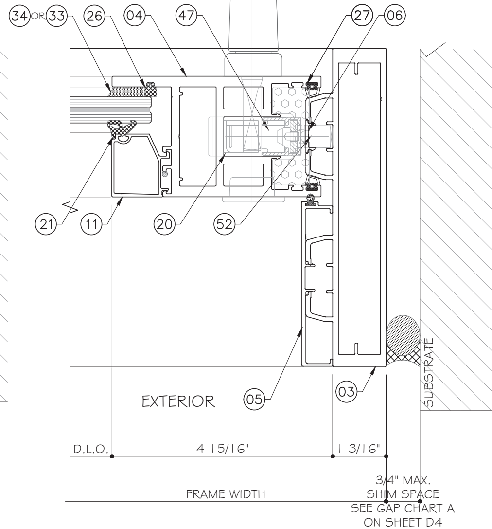
J D3 DETAIL
